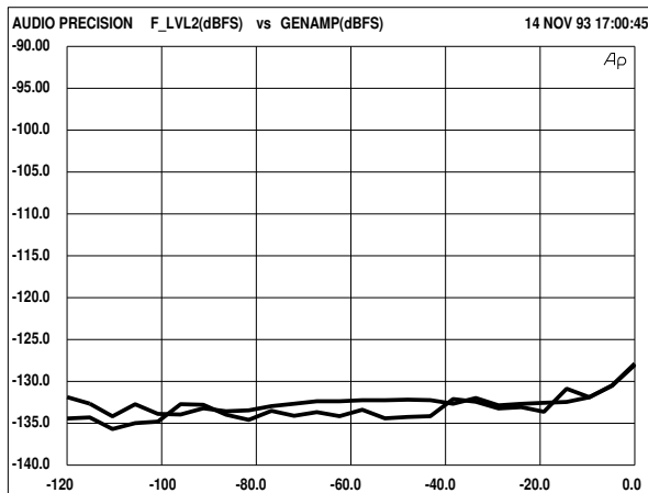
THD+N vs.level- 44.1k to 44.1k Conversion 1 kHz and 19 kHz tones
