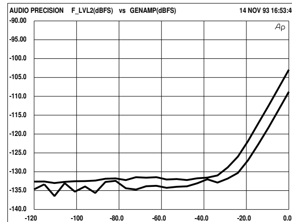
THD+N vs.level- 48k to 44.1k Conversion 1 kHz and 19 kHz tones
