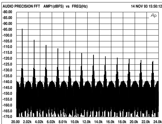
Fig. 7- 16 bit input signal -100 dB truncation by previous processing
